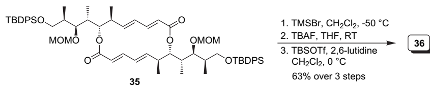
Scheme 10. Conversion of macrodilactone 35 into macrodiolide 36 .
