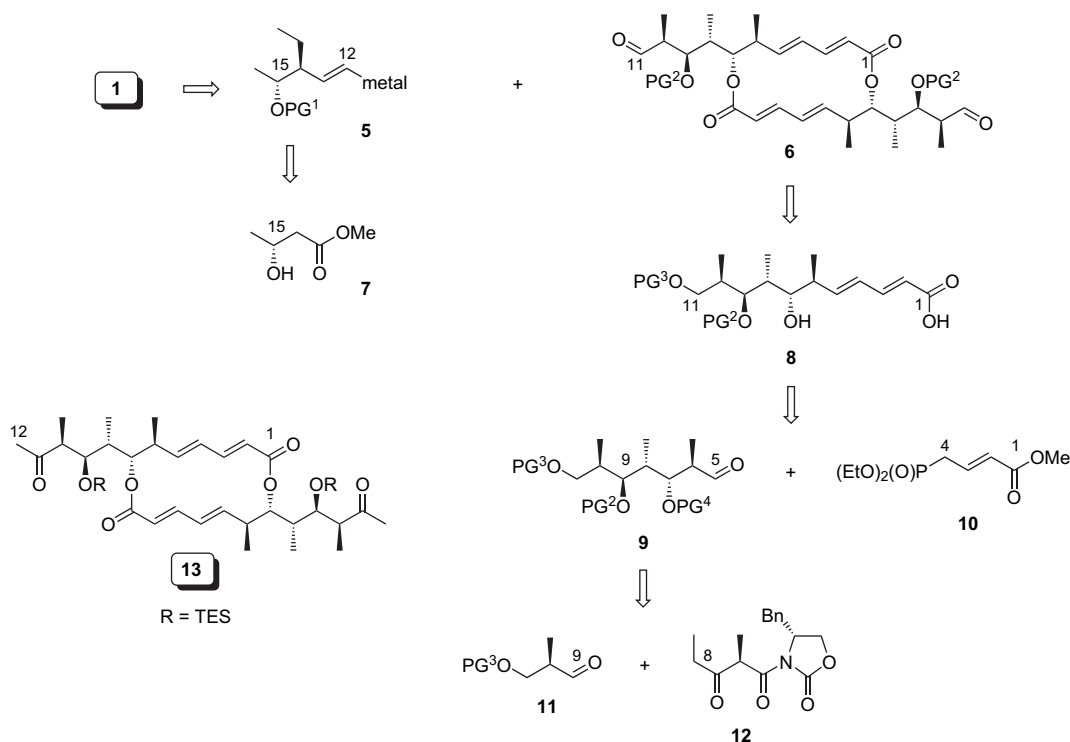
Scheme 2. Retrosynthetic analysis of efomycine M ( 1 ) and of elaiolide precursors 13 . PG=protecting group.
