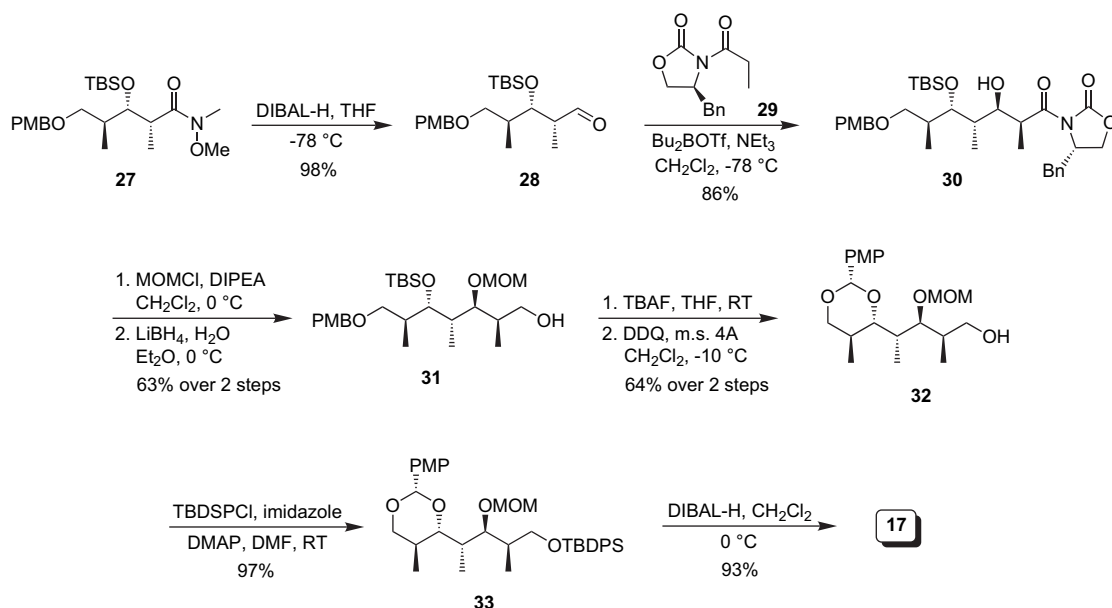
Scheme 5. Second generation synthesis of stereopentad 17 .
