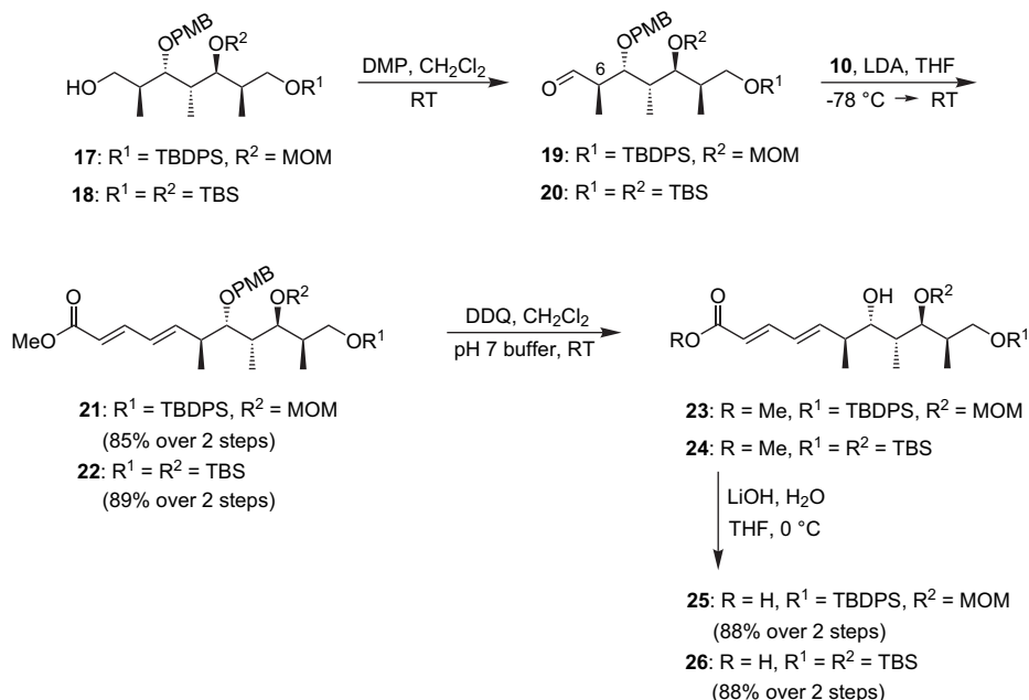
Scheme 4. Preparation of seco -acids 25 and 26 .
