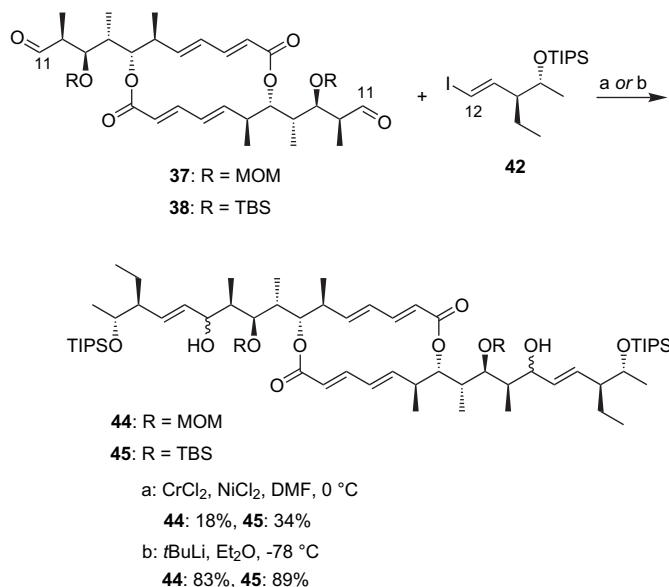
Scheme 8. Two-directional C11–C12 bond formation.
