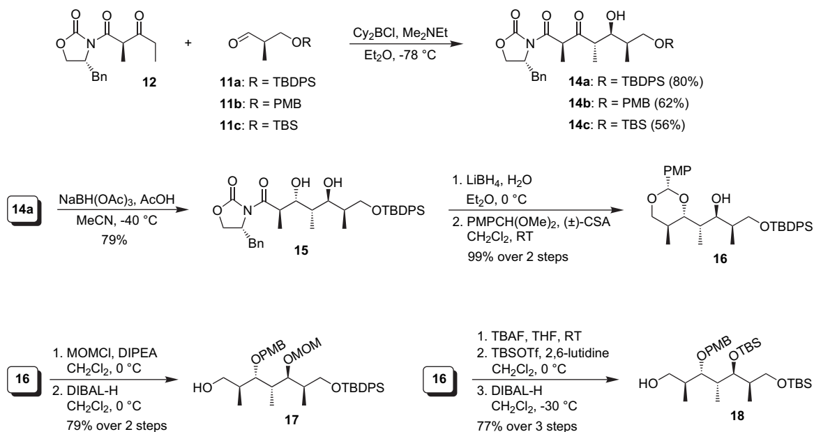
Scheme 3. Preparation of stereopentads 17 and 18 .
