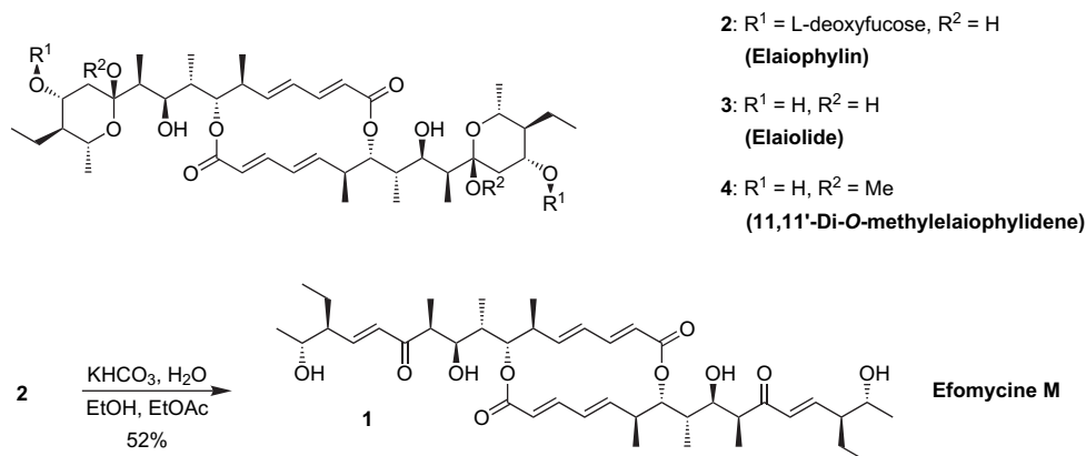
Scheme 1. Semi-synthetic origin of efomycine M ( 1 ) from elaiophylin ( 2 ) by base-catalyzed \beta -elimination.
