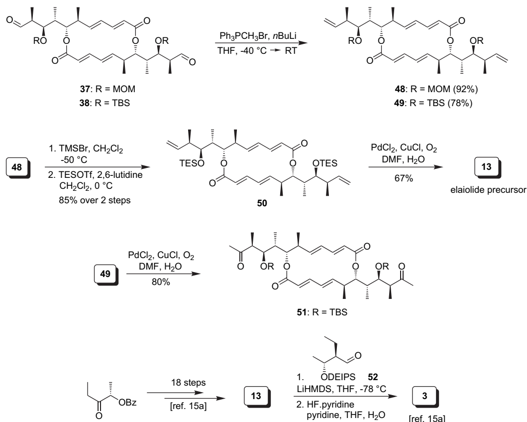
Scheme 12. Formal total synthesis of elaiolide (3) by a double Wacker oxidation.
