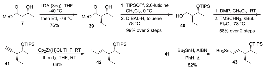
Scheme 7. Preparation of vinyl iodide 42 .
