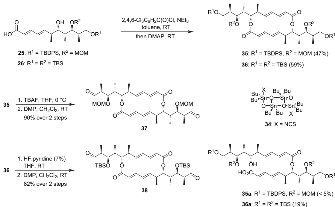
Scheme 6. Yonemitsu–Yamaguchi macrolactonization and preparation of bis-aldehydes 37 and 38 .
