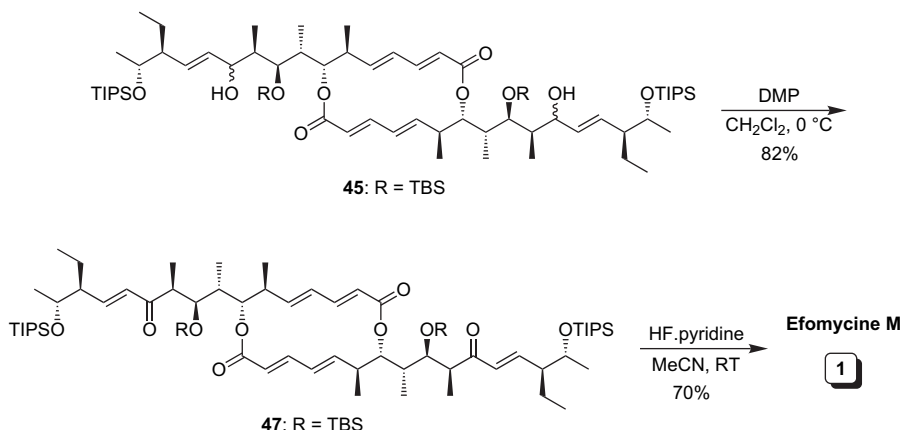
Scheme 11. Completion of the total synthesis of efomycine M ( 1 ).
