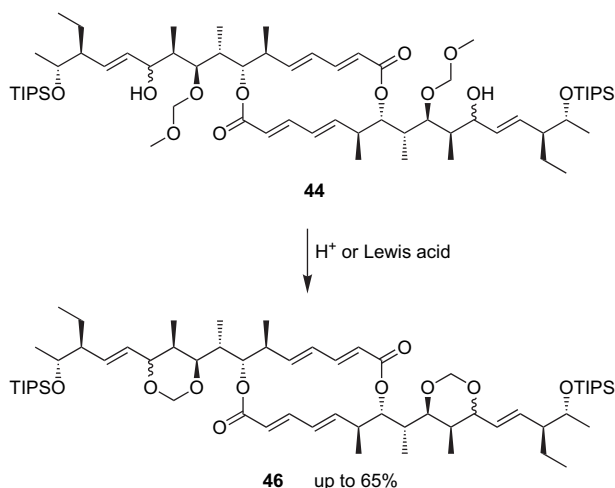
Scheme 9. Attempted cleavage of the MOM-protecting group.
